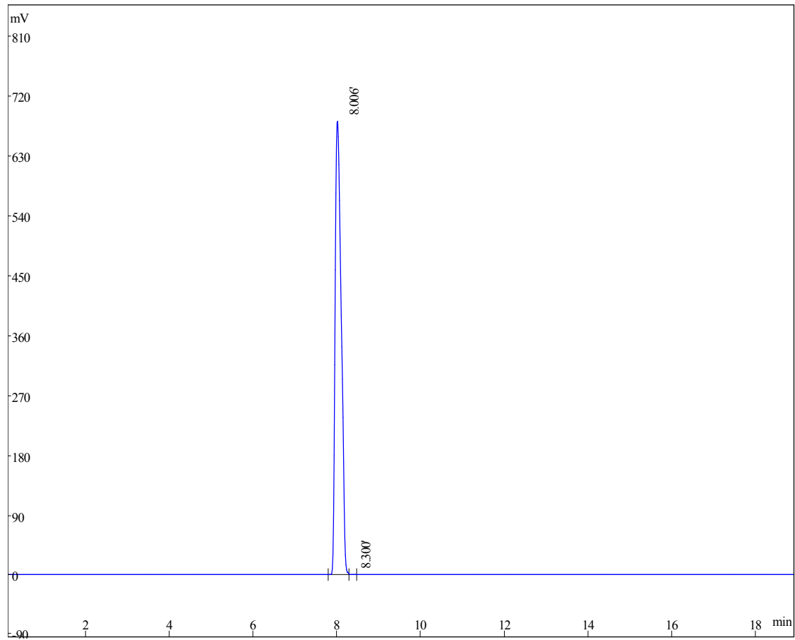
Chromatogram
